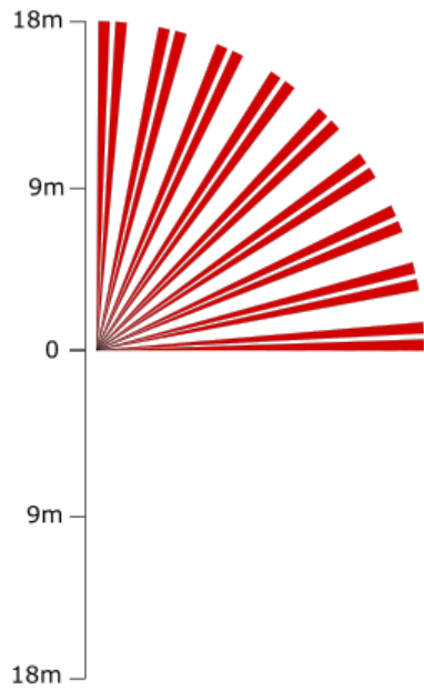
45° Bracket Mount
